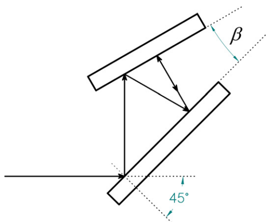
Figure 4. Schematic structure of a two-photodiode trap detector.
