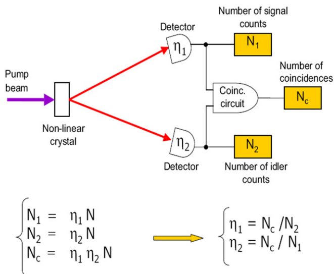
Figure 5. Scheme for absolute calibration of single-photon detectors.
