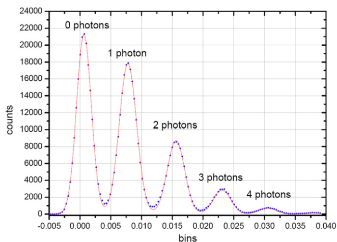
Figure 6. Typical distribution of the pulse amplitudes of single-photon events as detected by TES.
